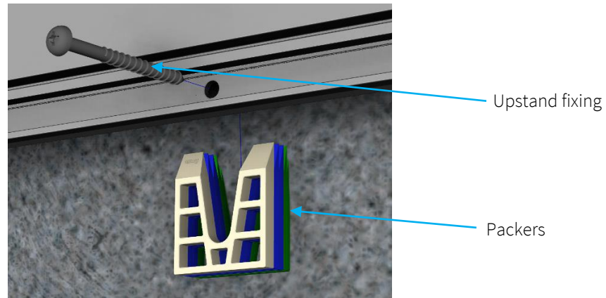
Figure 8 - Upstand fixings
