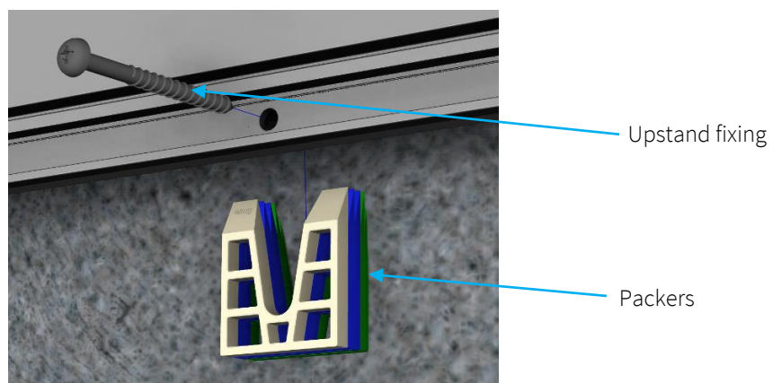
Figure 7 - Upstand fixings
