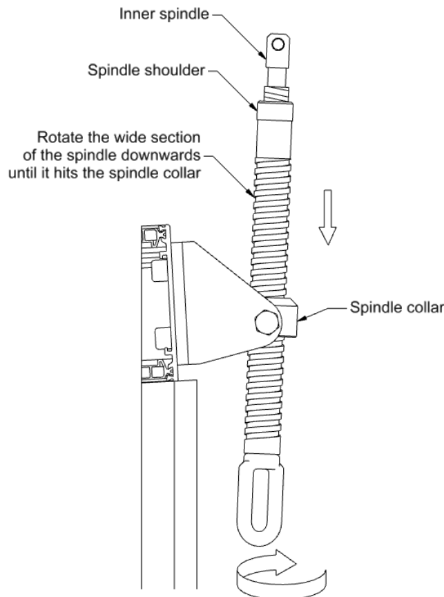
Figure 5 – Attach the spindle to the base bracket
