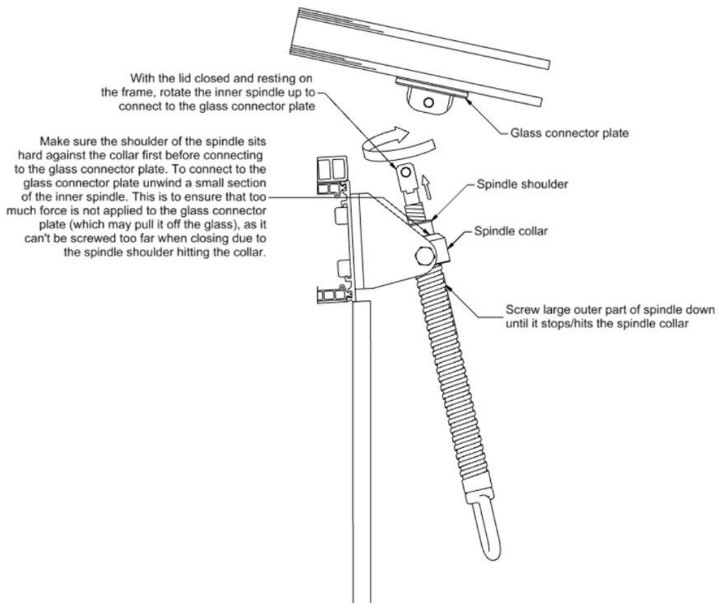
Figure 7 – Raise the inner of the spindle part and attach the spindle to the lid bracket
