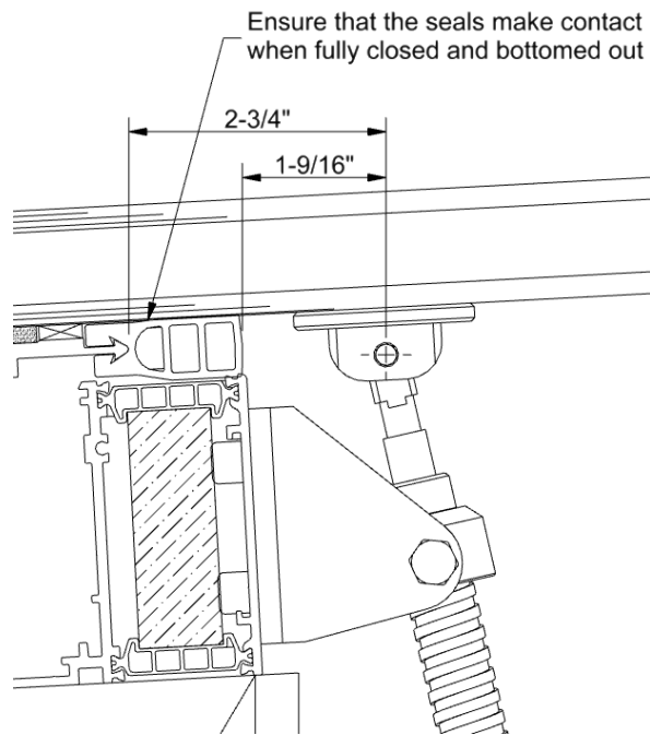
Figure 6 – Positioning of the lid bracket
