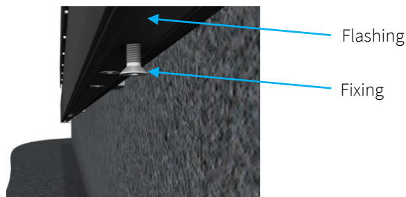
Figure 15 – Flashing fixings
