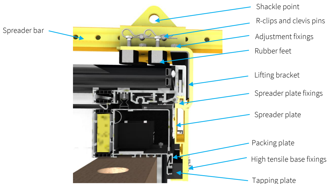
Figure 5 – Section showing bracket and framework
