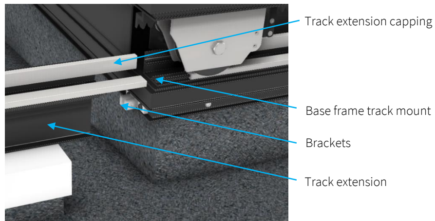
Figure 11 – Locating extension rails
