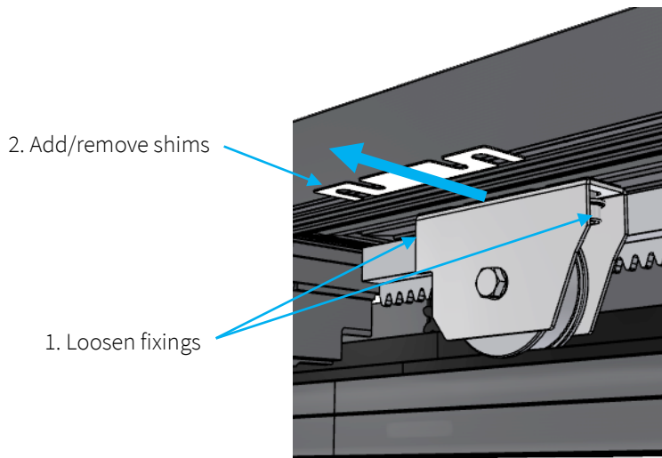
Figure 14 – Adjust lid position
