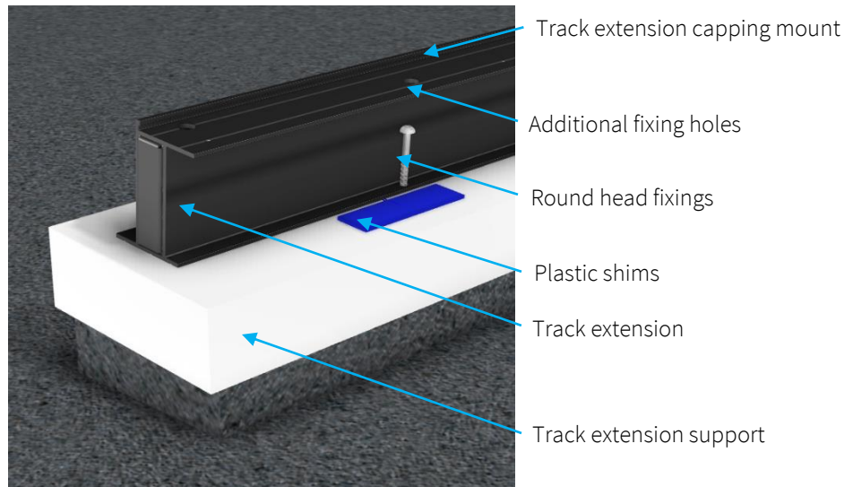
Figure 13 – Track extension fixings additional holes
