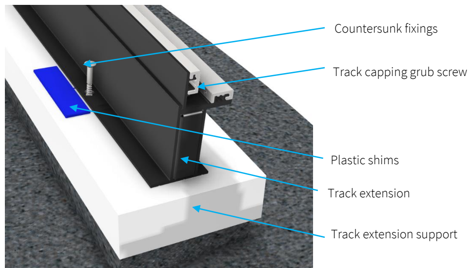
Figure 12 – Track extension fixings
