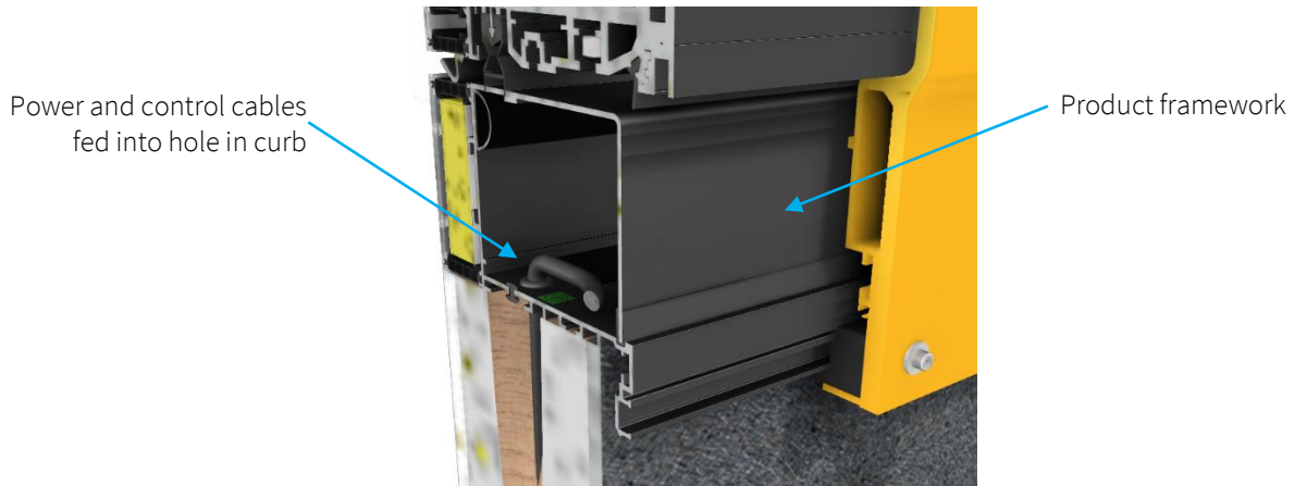
Figure 9 - Position of power and control cables in motor housing
