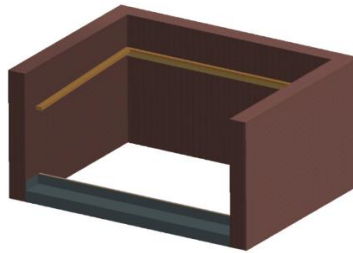
Figure 3 - Temporary wooden support battens in place
