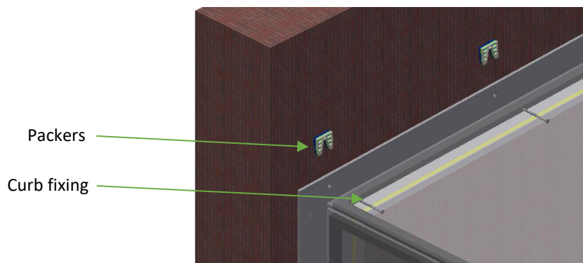
Figure 3 – Wall fixings
