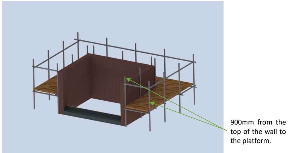
Figure 2 – Scaffolding arrangement
