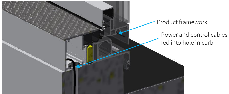
Figure 7 - Position of power and control cables in motor housing
