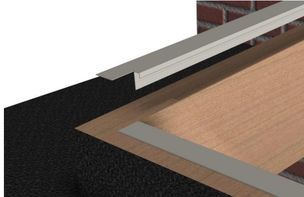
Figure 1 – Curb top trim placement
