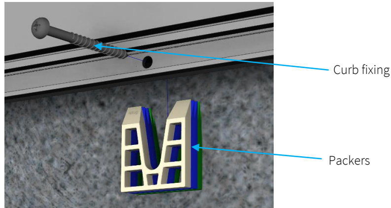
Figure 8 - Curb fixings
