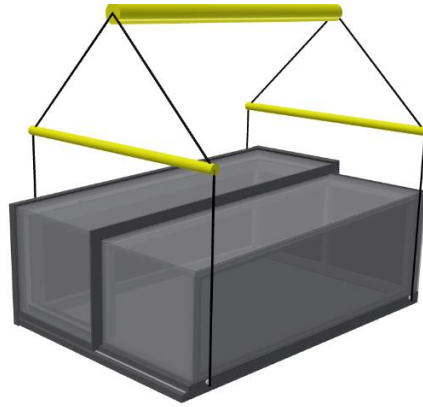
Figure 6 – Suggested lifting configuration
