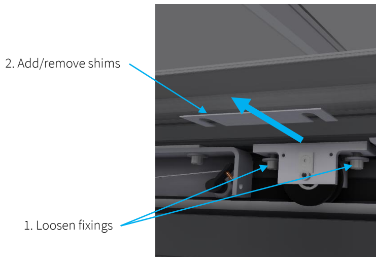
Figure 9 - Adjust door position
