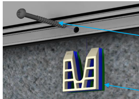
Figure 6 - Curb fixings
