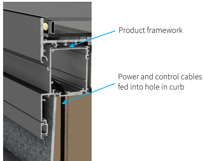
Figure 6 - Position of power and control cables in motor housing
