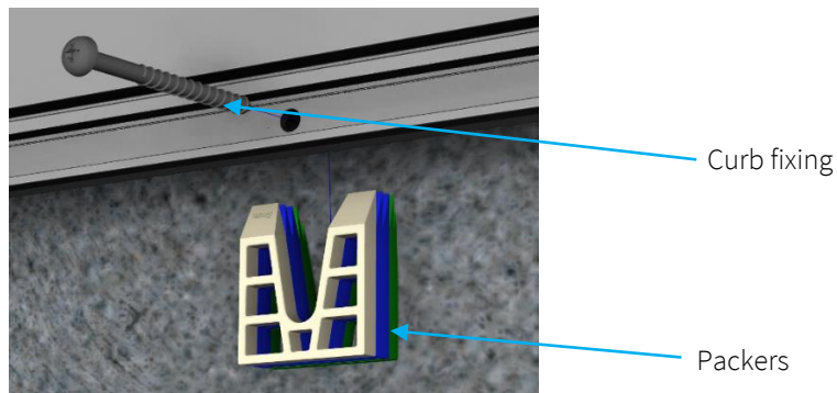
Figure 7 - Curb fixings
