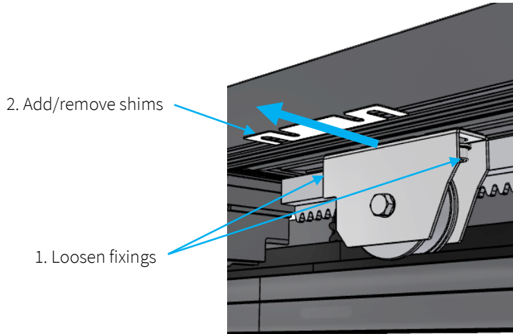
Figure 12 – Adjust lid position
