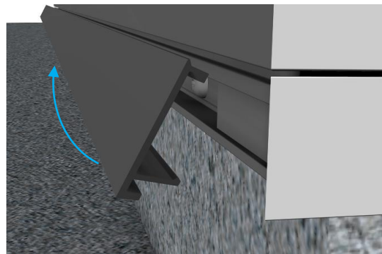
Figure 4 - Clip on cover
