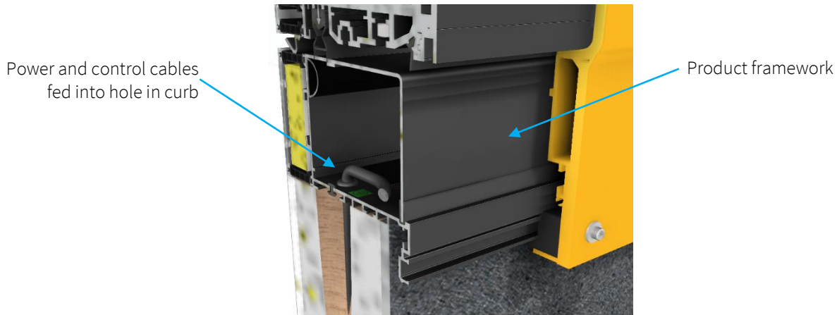
Figure 10 - Position of power and control cables in motor housing
