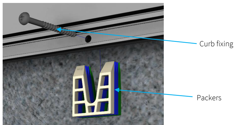
Figure 11 - Curb fixings
