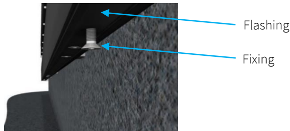
Figure 13 – Flashing fixings
