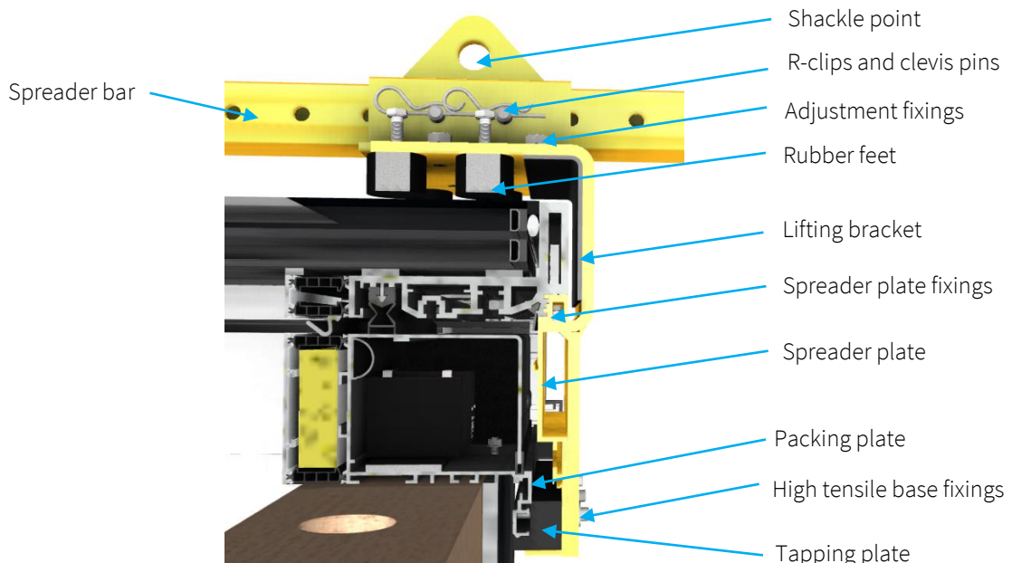
Figure 5 – Section showing bracket and framework
