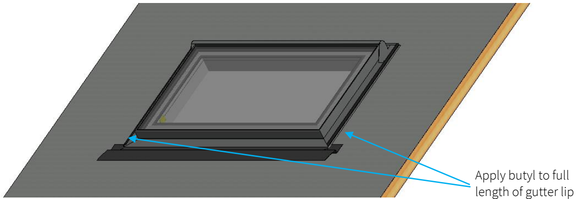
Figure 6a – Butyl tape applied to jambs
