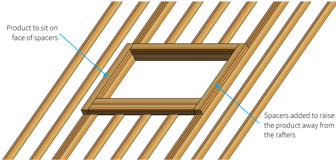
Figure C – Example of raised installation
