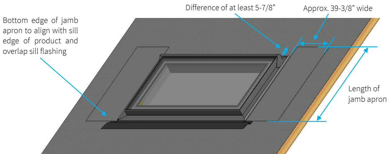
Figure 7a – Jamb aprons positioned
