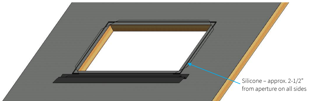
Figure 4b – Continuous silicone bead on top of underlay
