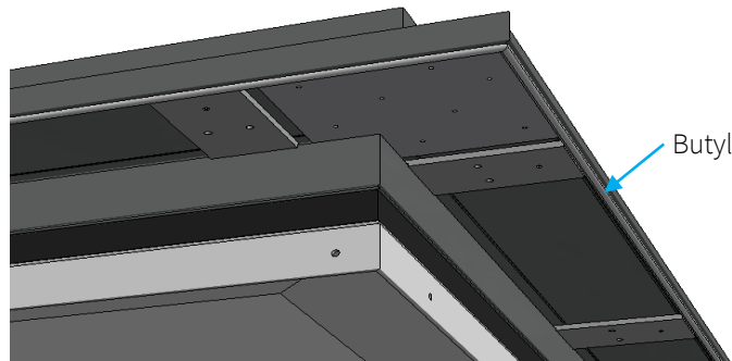
Figure 4c – Continuous butyl loop on the underside of the product
