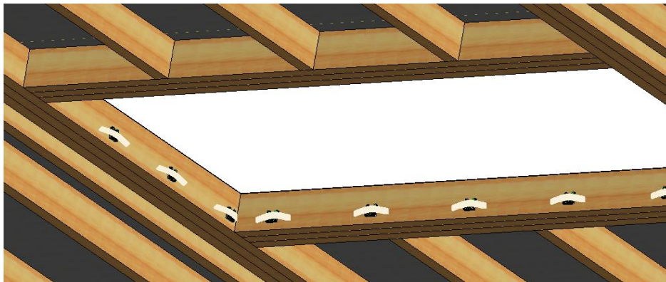
Figure 4a – Tape plastic packers along jambs and sill
