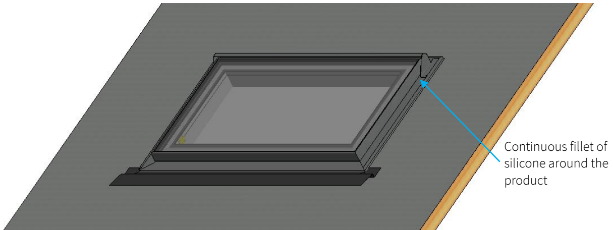
Figure 5 – Head, sill and jambs siliconed
