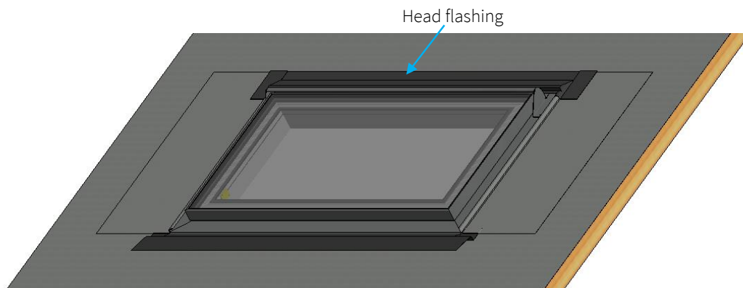
Figure 9a – Head flashing installed
