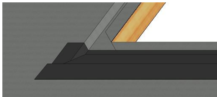
Figure 3b – Sill flashing detail for a sunken installation
