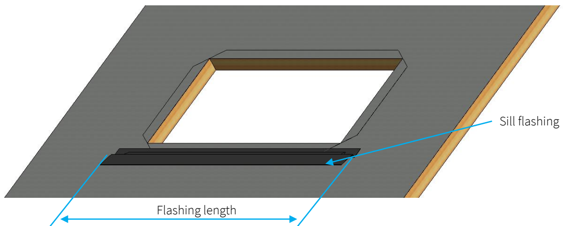
Figure 3a – Sill flashing in position
