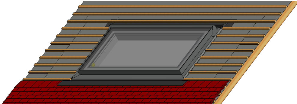
Figure 13a – Sill tiled and sill flashing finished
