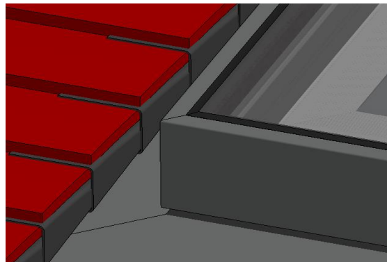
Figure 12a – Example of installed soakers
