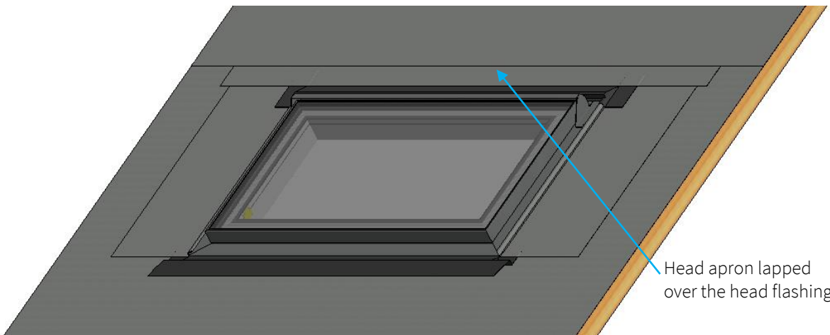
Figure 10 – Head apron installed
