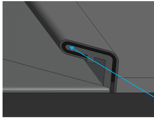
Figure 7b – Jamb apron adhered to butyl tape
